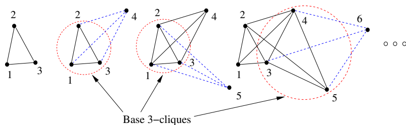
Figure 5.6: The process of constructing 3-trees.
